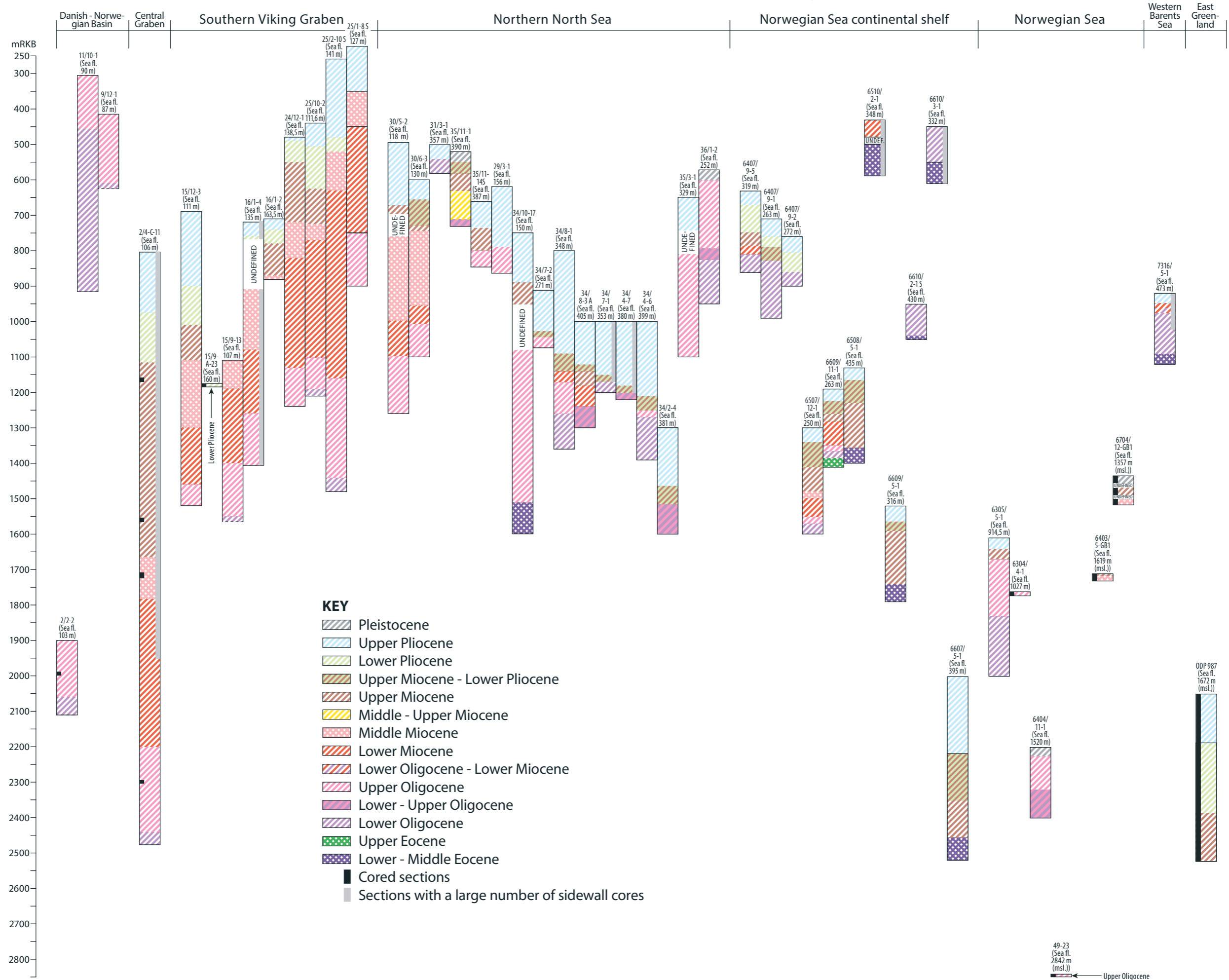
Diagram/Fig. 2: Chronostratigraphy of studied wells and boreholes. All depths are in metres below rig floor, except for the boreholes 6704/12-GB1 and 6403/5-GB1 and the core 49-23 which are in metres below mean sea level. The onshore Hjöllund and Rødding boreholes and the outcrop at Sarsbukta (Forlandsundet, Spitsbergen) in figure 1 are not included in this figure.
