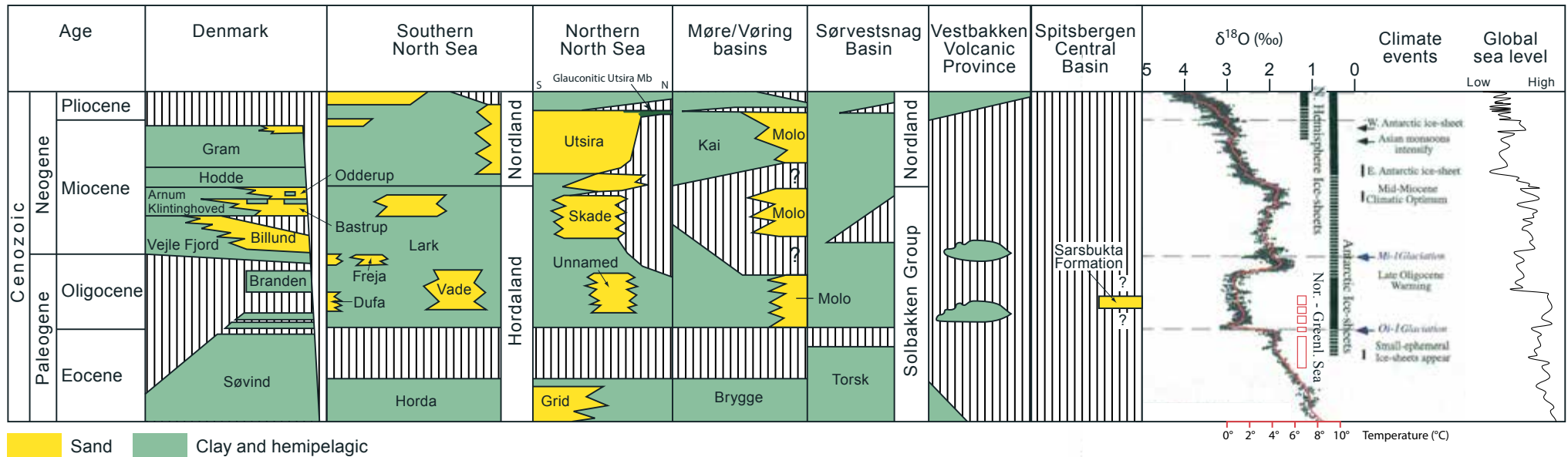
Fig. 5: General view of the Late Paleogene and Neogene lithostratigraphy in the investigated areas modified after Rundberg & Eidvin (2005), Rasmussen et al. (2008), and Eidvin et al. (2010 and work in progress). On the right-hand side of the diagram there is added some paleoclimatic data including a global deep-sea oxygen curve and periods with ice-sheets in the Antarctica and northern hemisphere (after Zachos et al. 2001) and a global sea level curve after Hardenbol et al. (1998). Periods with deposition of IRD at ODP Site 913 (off East Greenland) are also indicated (Eldrett et al. 2007).
