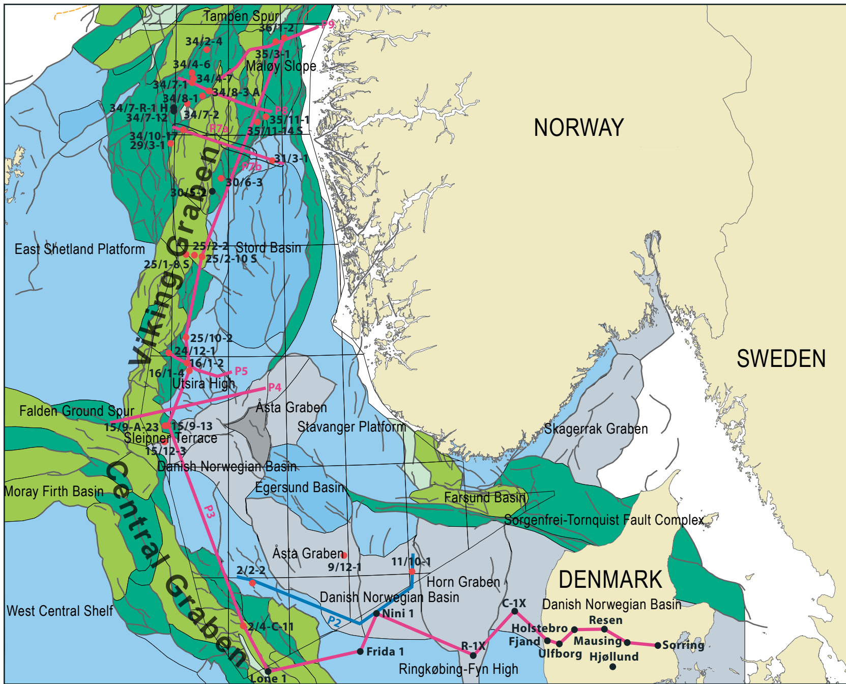
Fig.7: Map showing structural elements and seismic lines in the North Sea and Norwegian-Danish Basin. Red dots are investigated wells and boreholes, black dots are wells and boreholes referred to and magenta and blue lines are locations of seismic profiles. The map is according to the Norwegian Petroleum Directorate web page ( www.npd.no ). See Fig. 6 for legend.
