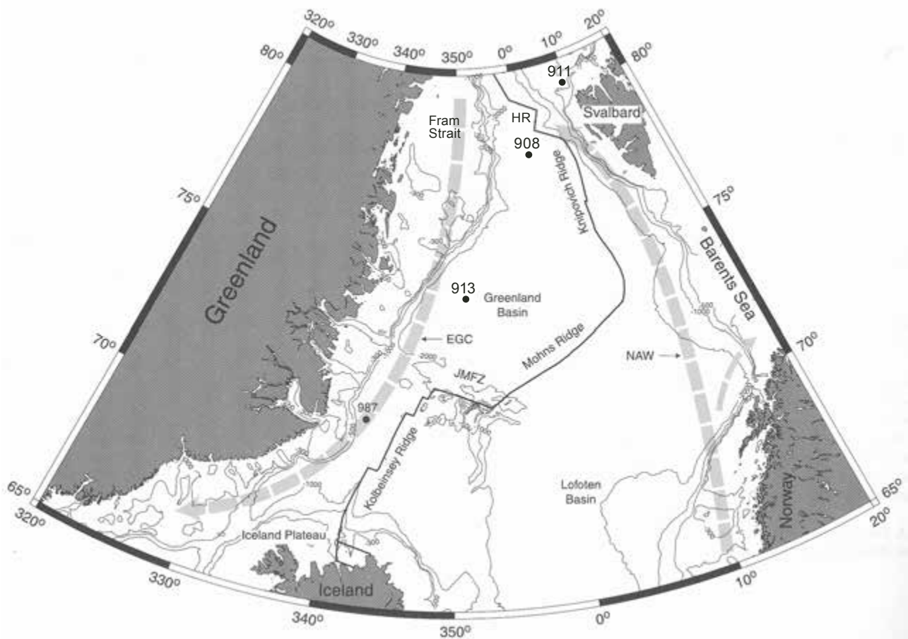
Fig. 8: Map of the Polar North Atlantic region with location of the ODP Sites 987, 913, 911 and 908. Bathymetry of the shelf and slope is shown. HR = Hovgård Ridge, EGC = East Greenland Current, JMFZ = Jan Mayen Fracture Zone, NAW = North Atlantic Water (modified after Butt et al. 2001).
