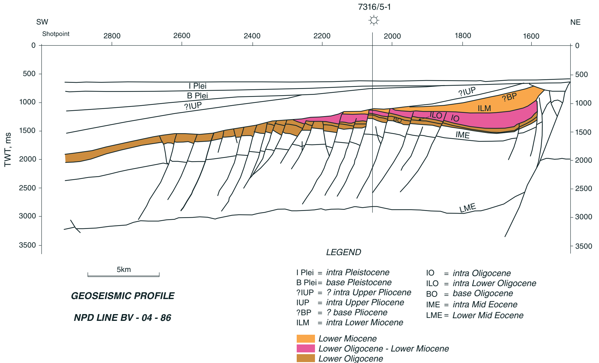
Profile. 15: Digitised seismic line NPD BV-04-86 (modified after Eidvin et al. 1998b).
